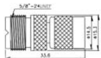
ATA01: TNC Plug to UHF Jack
