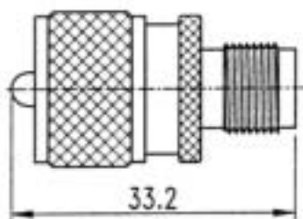
ATA02: TNC Jack to UHF Plug
