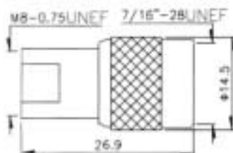
ATA00: TNC Plug to FME Plug
