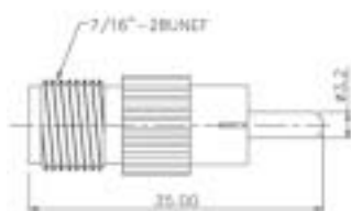
AT957: RCA Plug to TNC Jack
