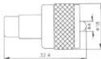
AT960: RCA Jack to UHF Plug
