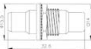
AT950: RCA Bulkhead Jack to Jack
