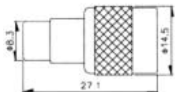
AT959: RCA Jack to TNC Plug
